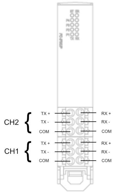
Modulo FC-IFSER Pin Out RS422
