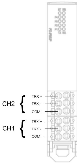
Modulo FC-IFSER Pin Out RS485
