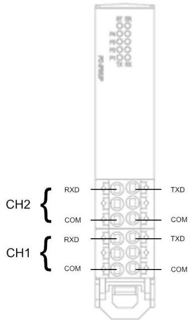
Modulo FC-IFSER Pin Out RS232
